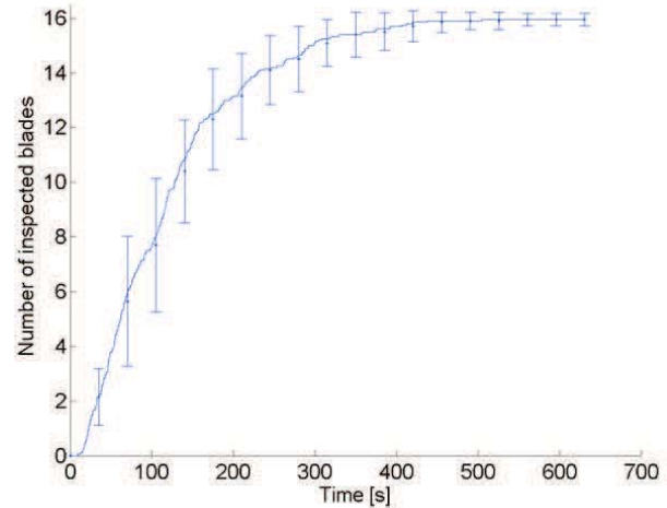
Fig. 12. Mean inspection progress over 20 experiments with 20 miniature robots inspecting a scenario with 16 objects.
