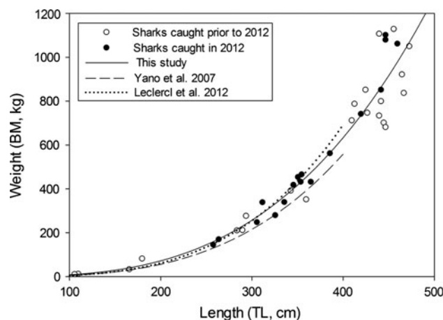
Fig. 2 Relationship between length and body mass (BM, kg). Open circles represent sharks caught prior to 2012 ( N = 23 ), and black-filled circles represent sharks caught in 2012 ( N = 17 ). The model of Leclerc et al. (2012) was based on fork length (FL, cm) and has been converted to total length (TL, cm) using the relationship described in this study
