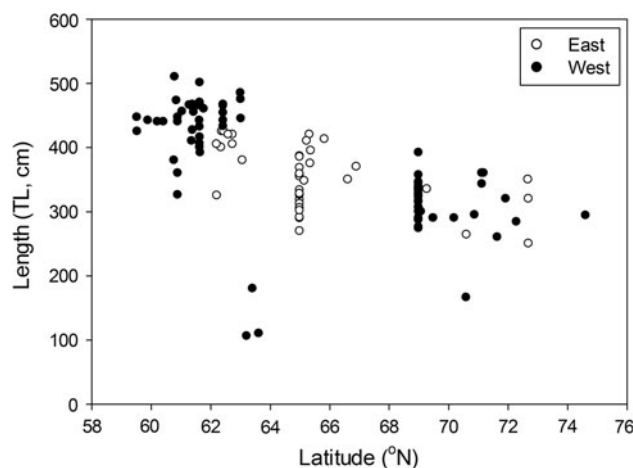
Fig. 4 Greenland shark length (TL, cm) at different latitudes ( N = 113 ). The largest sharks were caught at lower latitudes
